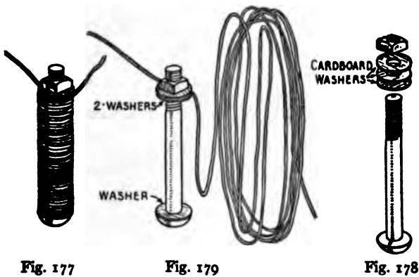
FIGS. 177-179. — The Electro-Magnet.
